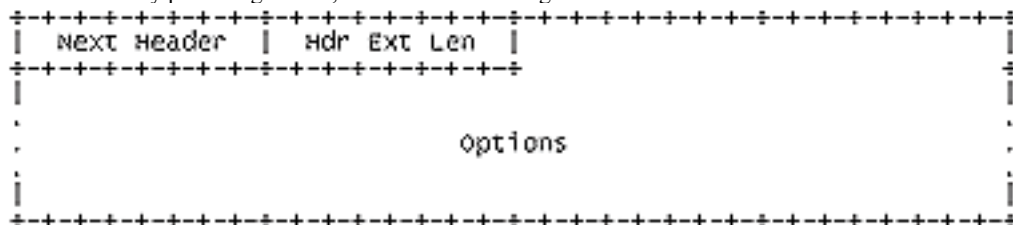
Next Header 8-bit selector. Identifies the type of header immediately following the Destination
